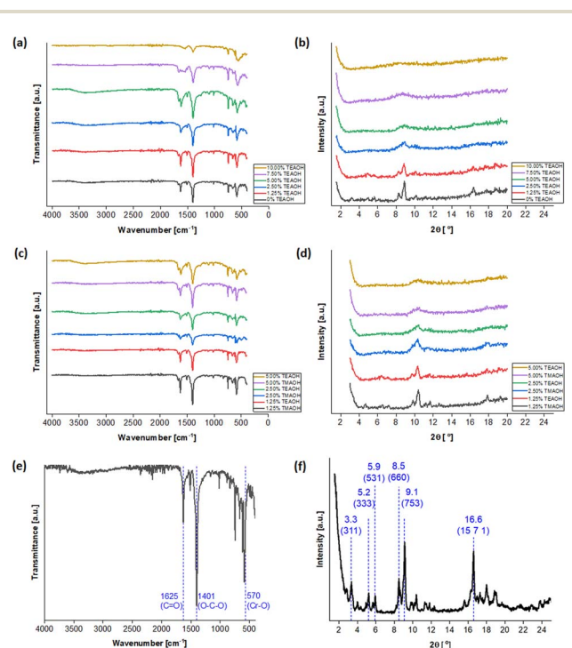
Fig. 3 Samples were prepared using different concentrations of TEAOH and were characterised by (a) ATR-FTIR and (b) PXRD. Spectra for the samples synthesised using 1.25%, 2.50% and 5.00% TEAOH solutions were also plotted against the (c) ATR-FTIR and (d) PXRD spectra of samples from 1.25%, 2.50% and 5.00% TMAOH solutions. Labelled peaks for the sample prepared from 1.25% TEAOH solution on the (e) ATR-FTIR and (f) PXRD spectra.
