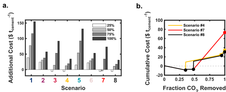
Fig. 4 (a) Additional costs to a cement plant ( \$ t_{\text{cement}}^{-1} ) to achieve up to net-zero CO 2 removal assuming \text{PSC} = \$60 t_{\text{CO}_2}^{-1} and \text{DAC} = \$200 t_{\text{CO}_2}^{-1} . The costs at 25%, 50%, 75%, and 100% removal are representative of actual costs that will be incurred by the cement manufacturing facility to achieve the desired CO 2 removal. (b) The total additional costs to a cement plant ( \$ t_{\text{cement}}^{-1} ) to achieve a fraction of CO 2 removal in Scenarios #4, #7, and #8. The dashed gray line at \$0 t_{\text{cement}}^{-1} represents the baseline costs.
