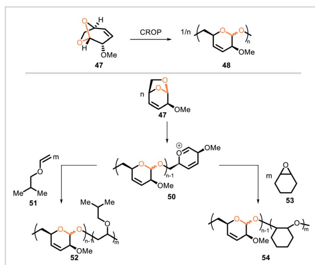
Scheme 8 Cationic ring-opening polymerization (CROP) of a levoglucosenone-derived monomer.
