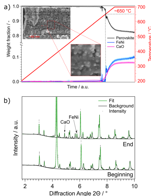
Fig. 6 (a) Weight fractions of NCF-Ni during a reduction ramp. The temperature was increased by a rate of 3 °C min -1 from 200 °C to 700 °C in H 2 /H 2 O atmosphere. At around 650 °C, a FeNi phase as well as a CaO phase started to form. This indicates the start of the exsolution process as well as the accompanied A-site segregation to compensate for the loss of B-site atoms. SEM images taken after the reduction experiments reveal nanoparticles with a diameter of around 60 nm, consistent with particles observed after reduction at 700 °C in lab-based experiments (Fig. 2c). (b) Comparison between the first and last diffractogram of the reduction. The emerging phases CaO and FeNi are marked.
