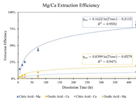
Fig. 4 Effect of dissolution time in 0.5 M citric and oxalic acid solutions on Mg and Ca extraction.
