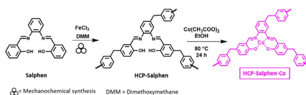
Fig. 2 Synthesis of catalyst HCP-Salphen-Co.
