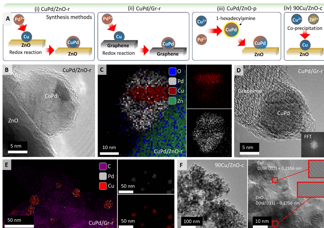
Fig. 1 (A) Schematics elaborating the synthesis of nanocatalysts through different methods, mainly (i) 5%Cu/Pd (3 : 2) over ZnO or (ii) graphene through the liquid reduction method, (iii) \text{Pd}^{2+} and \text{Cu}^{2+} reduction with ethylene glycol, stabilization with 1-hexadecylamine and deposition on ZnO to obtain CuPd/ZnO-p, and (iv) 90% Cu with Zn nitrates, reduced with aqueous \text{Na}_2\text{CO}_3 to produce 90Cu/ZnO-c (for the details of synthesis see the Experimental section), (B) HRTEM image of the bimetallic CuPd/ZnO-r catalysts, (C) corresponding EDX mapping showing the distribution of 'Pd', 'Cu' and 'O' atoms in CuPd/ZnO-r, (D) HRTEM image of the CuPd/Gr-r catalysts, (E) EDX mapping showing the distribution of 'C', 'Pd', and 'Cu' atoms in CuPd/Gr-r and (F) HRTEM image of the 90Cu/ZnO-c catalysts, also showing the interplanar spacing of Cu ( d = 0.256 nm) and ZnO ( d = 0.277 nm).
