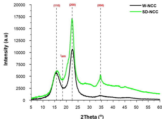
Fig. 4 XRD spectra of W-NCC and SD-NCC.
