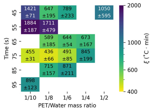
Fig. 6 Effect of batch holding time and m_{\text{PET}}/m_{\text{w}} on the environmental energy impact metric from fast hydrolysis of post-consumer PET at T_{\text{SP}} = 510 °C.
