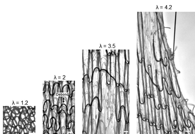
Fig. 5 Snapshots of a knit-PCU composite stretched under an optical microscope. Scale bars are 200 \mu\text{m} .
