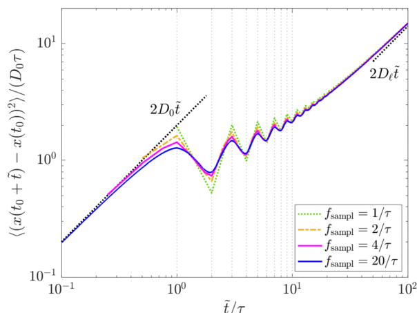
Fig. 3 Analytic result for the MSD of a single particle in an attractive harmonic feedback potential ( \frac{\kappa}{\gamma}\tau = 2.0 ) and different sampling rates f_{\text{sampling}} (= number of measurements of the particle position per delay time \tau ) of the particle position. We find a decrease in the MSD compared to free diffusion (as indicated by the black line 2D_0\tilde{t} at short times) and oscillations whose period is set by 2\tau which arise as the particle is being pulled back to its past position. At long times the particle shows diffusion with a reduced diffusion constant D_\ell < D_0 . Discrepancies appear in the MSD for small sampling rates as these do not cover the full average over t_0 . A high sampling rate is thus necessary to obtain the “correct” MSD.
