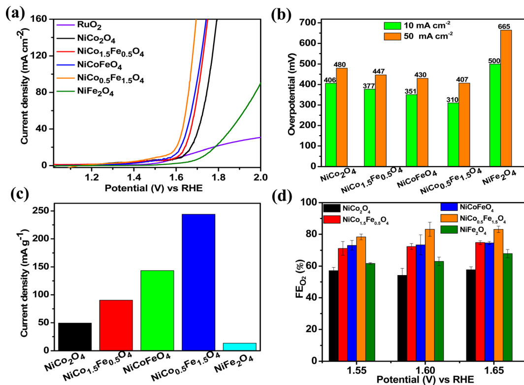
Fig. 5 (a) LSV polarization plots; (b) overpotential at 10 and 50 mA cm -2 current densities; (c) mass activities, and (d) FE(%) of oxygen evolution over the synthesized catalysts.
