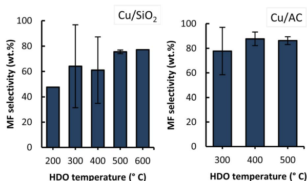
Fig. 8 Averaged MF selectivity in furanics obtained from molten salt hydro-pyrolysis of pinewood and subsequent hydrodeoxygenation with Cu/SiO 2 (left) and with Cu/AC (right) as a function of catalyst bed temperature. Conditions: 0.4 MPa and hydro-pyrolysis at 350 °C.
