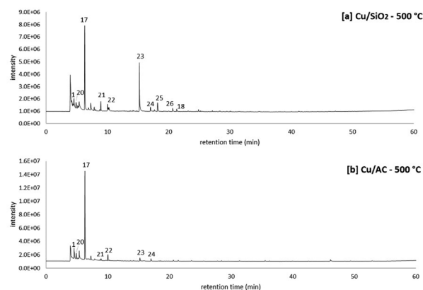
Fig. 6 Molten salt hydropyrolysis of pinewood at 350 °C and hydrodeoxygenation at 500 °C with Cu/SiO 2 (top chromatogram) and with Cu/AC (bottom chromatogram) at 0.4 MPa. Pyrograms correspond to the 2nd series of experiments.
