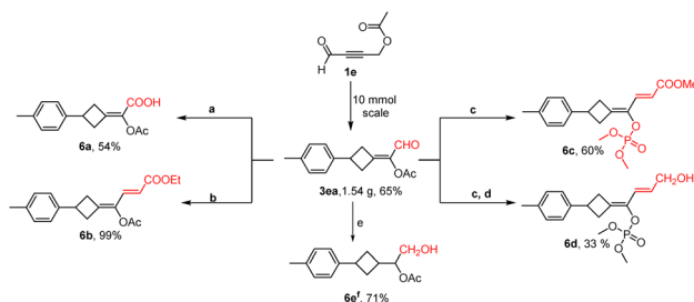
Scheme 4 Gram-scale reaction and synthetic applications. (a) \text{NaOCl} (3.0 eq.), \text{NaH}_2\text{PO}_4 (4.0 eq.), 2-methyl-2-butene/ \text{tBuOH}/\text{H}_2\text{O} (3/3/1). (b) \text{Ph}_3\text{PCHCOOEt} (1.2 eq.), DCM. (c) \text{NaH} (1.2 eq.), (\text{MeO})_2\text{POCHCOOEt} (1.2 eq.), THF. (d) \text{DIBAL-H} (1.1 eq.), toluene, -78^\circ\text{C} . (e) \text{NaBH}_4 (3.0 eq.), \text{CH}_3\text{OH} . (f) Four isomers were observed in the NMR spectra.
