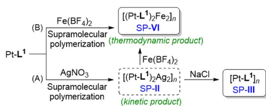
Scheme 1 Proposed formation mechanism of SP-II, SP-III and SP-VI in the presence of secondary metal ions: (A) AgNO 3 and (B) Fe(BF 4 ) 2 , upon the addition of NaCl or Fe(BF 4 ) 2 to SP-II.
