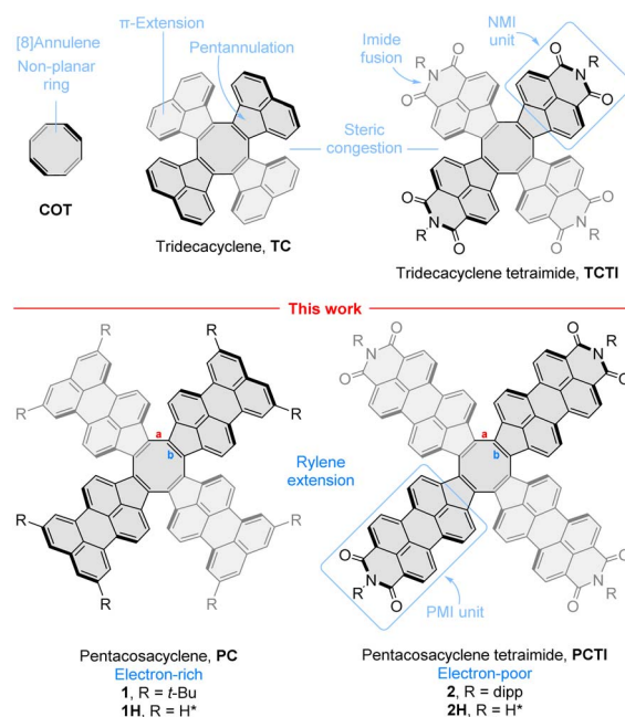
Fig. 1 Cyclooctatetraene and its radially π-extended analogues. Bond labeling is indicated for pentacosacyclene derivatives. dipp, 2,6-diisopropylphenyl.
