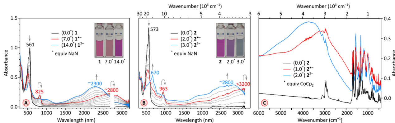
Fig. 5 (A) Stepwise reduction of 1 (0.154 mM in THF) with sodium naphthalenide (NaN, 1.54 mM in THF). The red and blue traces correspond to the maximum concentration of [1]^{1-} and [1]^{2-} , respectively. (B) Stepwise reduction of 2 (0.10 mM in THF) with sodium naphthalenide (NaN, 1.0 mM in THF) in the presence of 15 crown 5 ether (100 equiv.). The red and blue traces correspond to the maximum concentration of [2]^{1-} and [2]^{2-} , respectively. (C) IR spectra in a KBr pellet of reduction of 2 with cobaltocene (in THF). The black, red and blue traces correspond to the maximum concentration of 2 , [2]^{1-} and [2]^{2-} , respectively.
