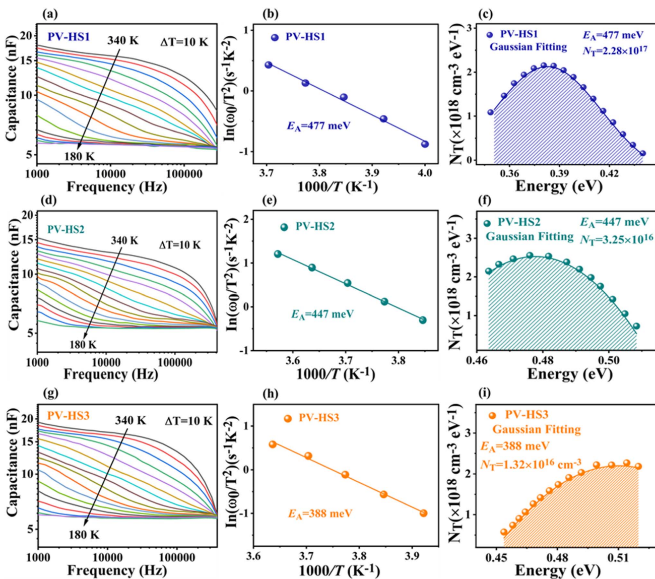
Fig. 6 Characterization of temperature-dependent admittance spectroscopy for Sb 2 (S,Se) 3 photovoltaic devices. (a, d and g) Variation of capacitance at different frequencies and temperatures. (b, e and h) Using the Arrhenius plots of the characteristic frequencies to acquire the defect activation energy. (c, f and i) Defect distributions of PV-HS1, PV-HS2 and PV-HS3 devices.
