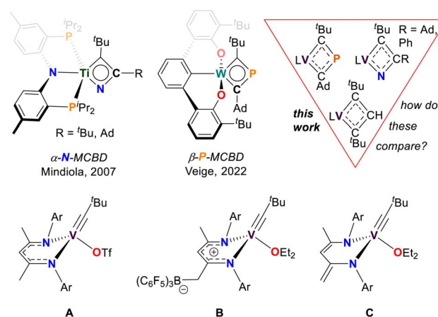
Fig. 1 Top: Isolable pnictogen-based metallacyclobutadienes (MCBD) complexes and the vanadacyclobutadiene (VCBD) species reported in this work ( L = dBDI^{2-} ). Bottom: Selected [V] alkyidyne complexes, with complex C being the focus of the present study.
