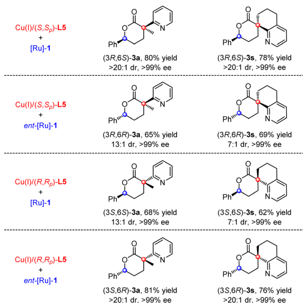
Scheme 2 Stereodivergence demonstration.
