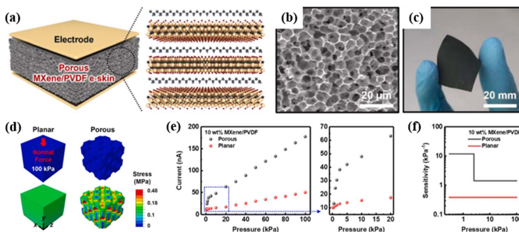
Fig. 12 (a) Schematic diagram showing the porous MXene/PVDF e-skin. (b) SEM image of the highly flexible porous MXene/PVDF e-skin. (c) Photograph of the highly flexible porous MXene/PVDF e-skin. (d) FEA of planar and porous structures and stress distribution under 100 kPa. (e) Comparison of piezoelectric sensing performance between porous- and film-structured 10 wt% MXene/PVDF e-skins. (f) Piezoelectric sensitivity analysis of porous- and film-structured MXene/PVDF e-skins. This figure has been reproduced from ref. 27 with permission from Elsevier, copyright 2021.
