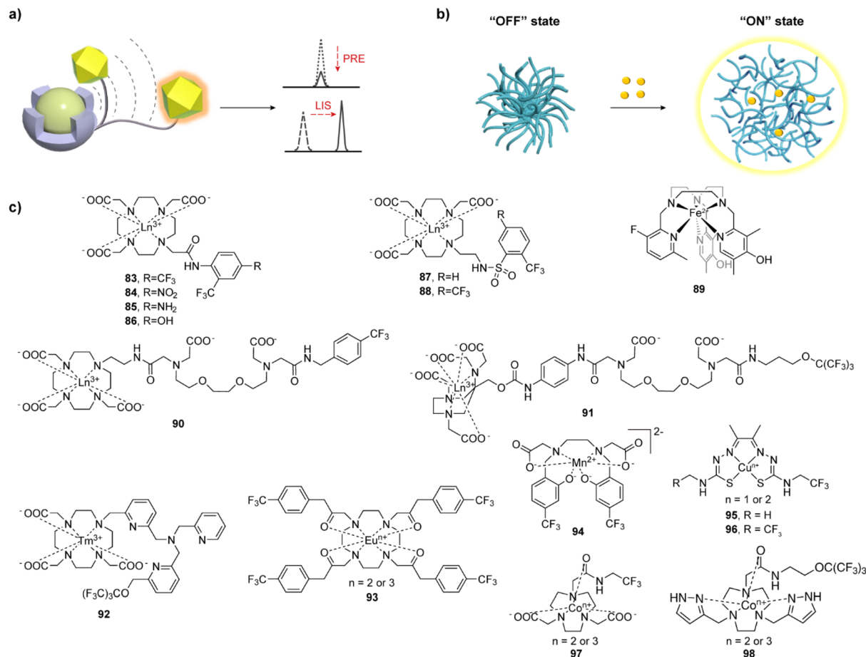
Fig. 12 The most common mechanisms used for preparation of responsive fluorinated MRI probes. (a) The design principle that uses a chelate with the paramagnetic lanthanide or transition metal ion (green ball) covalently bound to a fluorinated functional group (yellow polyhedron). The effect of paramagnetic metal ions on fluorine atoms varies depending on the distance, leading to changes in ^{19}\text{F} MR signals: at shorter distances, T_1 and T_2 relaxation times are shortening (PRE) or ^{19}\text{F} NMR frequency changes (LIS). (b) Fluorinated bioresponsive nanoprobe utilizes the principle in which the low ^{19}\text{F} MRI signal exists in assembled nanoprobe due to the significant T_2 shortening (left), which, in the presence of the analyte, triggers the NP disassembly and hence an enhanced ^{19}\text{F} MRI signal (right). (c) The structures of fluorinated bioresponsive probes 83 – 98 , which take advantage of PRE or LIS effect.
