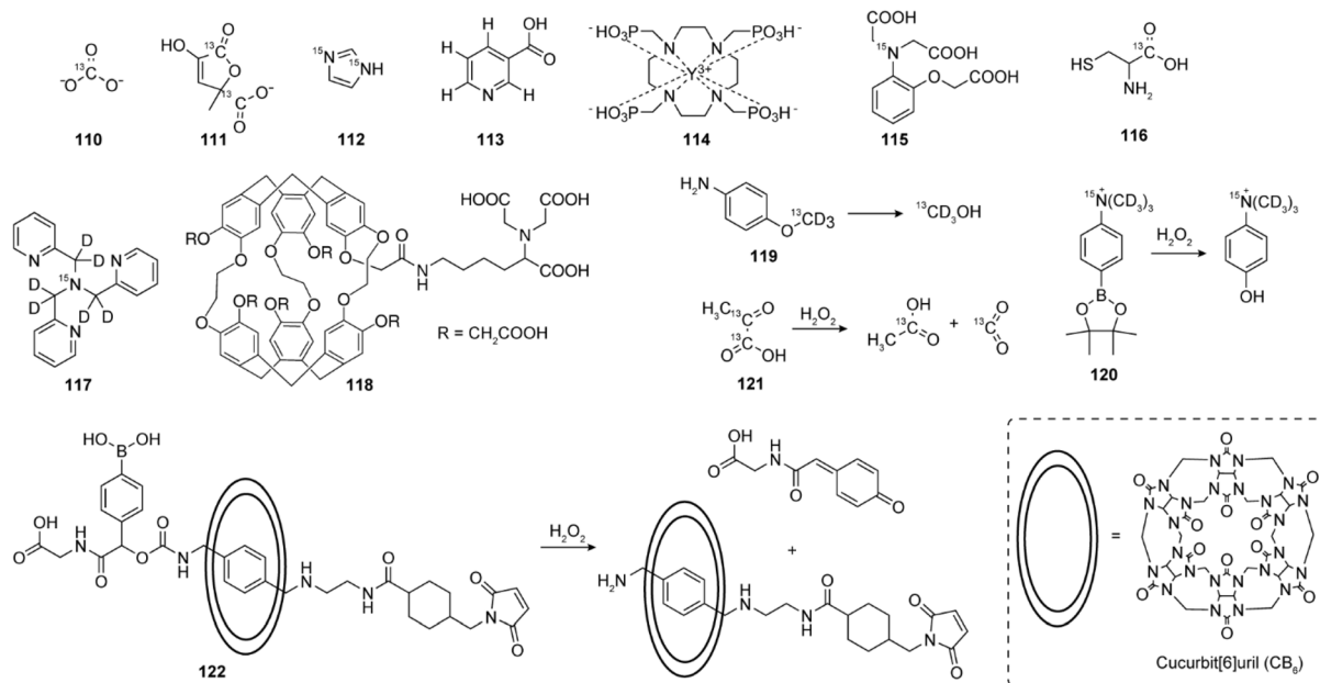
Fig. 14 The representative HP probes that are sensitive to pH ( 110–114 ), Ca(II) ( 115 ), Zn(II) ( 116–118 ), HOCl ( 119 ) and \text{H}_2\text{O}_2 ( 120–122 ). These presented probes contain either ^3\text{He} , ^{13}\text{C} , ^{15}\text{N} , ^{89}\text{Y} or ^{129}\text{Xe} nuclei to generate HP signal. The following techniques were employed for the signal amplification: dDNP for probes 110–111 , 114–117 and 119–120 ; SABRE for probes 112–113 and 121 ; SEOP for probes 118 and 122 .
