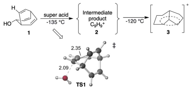
Scheme 1 Previous experiments on C_9H_9^+ cations. 50 The transition state TS1 is visualized using CYLVview 1.0 , 51 with key bond lengths labeled in Å. The C–O bond breaks first, and the C–C bond formation occurs subsequently in an asynchronous manner (see ESI† for details).
