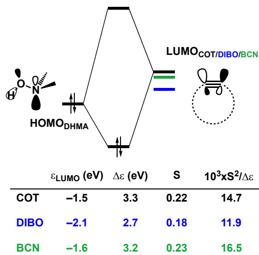
Fig. 3. Schematic diagrams with LUMO energies, energy gaps \Delta\epsilon , overlaps S , and values of S^2/\Delta\epsilon term associated with the key donor–acceptor interaction between \text{HOMO}_{\text{DHMA}}|\text{LUMO}_{\text{alkyne}} along with the retro-Cope elimination reactions between cyclooctyne ( COT ), DIBO and BCN with DMHA . All were computed at the consistent geometries where the length of the \text{C}\cdots\text{H} bond is 1.50 Å at ZORA-BP86/TZ2P.
