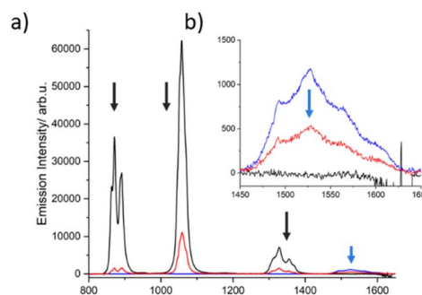
Fig. 6 Emission spectra ( \lambda_{\text{exc}} = 400 nm) of iso-absorbant solutions of complexes ( 1 ) (black trace), ( 2 ) (blue trace), and ( 3 ) (red trace) in MeOH- d_4 : DMSO- d_6 (1 : 1) solution at room temperature (a) with the corresponding \text{Er}^{3+} emission zoom (b).
