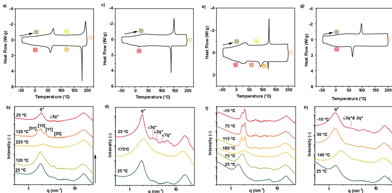
Fig. 5 (a, c, e and g) DSC traces of NPDIs 1 (a), 2 (c), 3 (e) and 4 (g) obtained with a rate of 5 K min -1 . Colored squares correspond to the different phases observed. (b, d, f and h) 1D transmission scattering profiles at different temperatures of 1 (b), 2 (d), 3 (f) and 4 (h).
