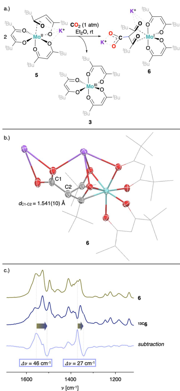
Fig. 6 (a) Reaction of 5 upon exposure to \text{CO}_2 . (b) XRD solid state structure of 6 . (c) IR-spectrum of 6 (green), ^{13}\text{C}\text{6} (dark blue) and the corresponding subtraction spectrum (light blue).
