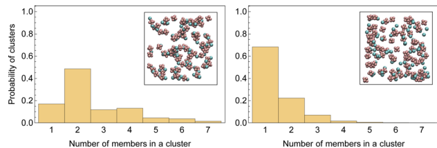
Fig. 3 Histograms of sizes of randomly picked clusters in \text{LiPF}_6 in DMC (left) and \text{LiPF}_6 in DMC/EC (right). The inlaid images show an arbitrary snapshot of ion clusters.
