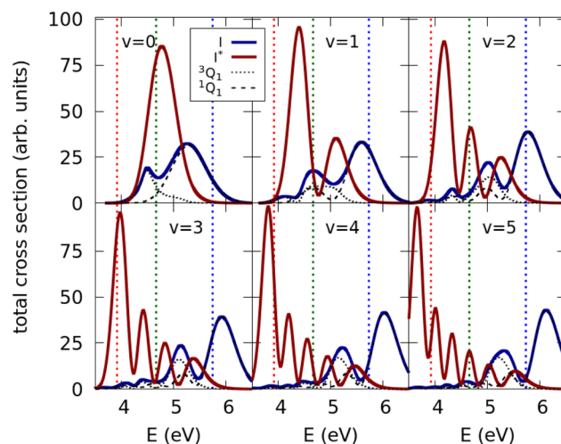
Fig. 2 Theoretical absorption spectra of \text{CH}_3\text{I} for the initial vibrational states v = 0 –5 of the \text{CH}_3 –I stretching mode. The absorption spectra calculated for the ^3Q_0 (red thick solid line), ^1Q_1 (black dashed line), and ^3Q_1 (black short-dashed line) states are shown in the figure for the six first vibrational states v = 0 –5 of the \text{CH}_3 –I stretching mode. The sum of the ^1Q_1 and ^3Q_1 spectra, that corresponds to the I fragment channel, is also displayed (blue thick solid line). The three vertical lines mark the energies corresponding to the excitation wavelengths of 316 nm (3.92 eV; red line), 266 nm (4.66 eV; green line), and 216 nm (5.74 eV; blue line).
