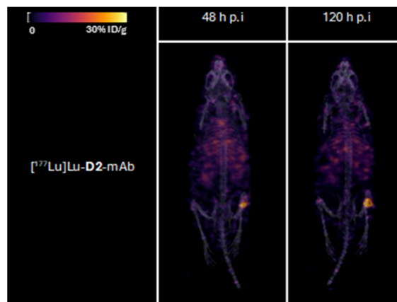
Fig. 9 Representative 3D maximum intensity projections for all mice ([ 177 Lu]Lu-D2-mAb) in 177 Lu SPECT/CT imaging cohort at 48 and 120 h post-injection. Signal normalised to same thresholding (% ID g -1 ).
