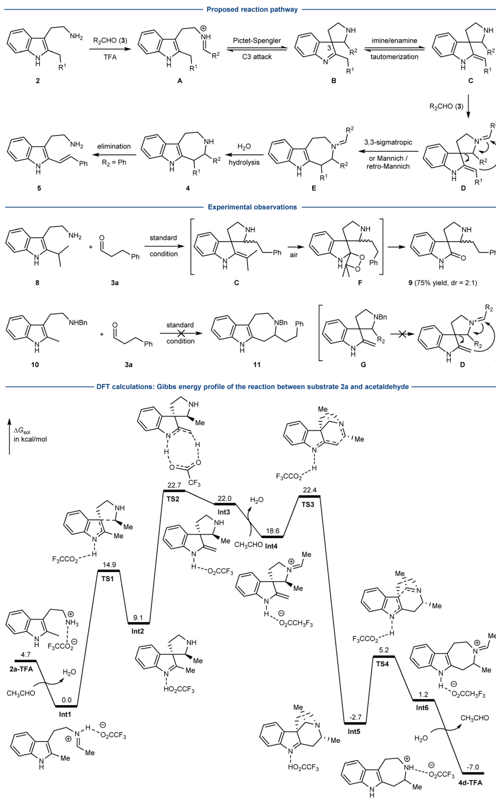
Scheme 3 Reaction mechanism.
