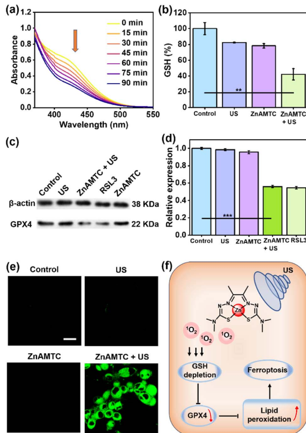
Fig. 3 Ferroptosis induction by ZnAMTC under US irradiation. (a) Irradiation-time-dependent GSH (200 μM) depletion by ZnAMTC (50 μM) upon US irradiation at 298 K. (b) GSH levels in 4T1 cells after different treatments. Data are shown as mean \pm SD ( n = 4 ). Statistical significance was calculated using a two-tailed Student's t -test, * p < 0.05 , ** p \leq 0.01 or *** p \leq 0.001 . (c) Western blot analysis of GPX4 in 4T1 cells after different treatments. (d) Relative expression levels of GPX4 calculated from (c). Data are shown as mean \pm SD ( n = 4 ). Statistical significance was calculated using a two-tailed Student's t -test, * p < 0.05 , ** p \leq 0.01 or *** p \leq 0.001 . (e) Fluorescence images of 4T1 cells stained with C11-BODIPY after different treatments. C11-BODIPY: \lambda_{\text{ex}} = 488 nm; \lambda_{\text{em}} = 570 \pm 50 nm; scale bar: 20 μm; US irradiation: 1.0 MHz, 3 W cm ^{-2} , 10% duty cycle, 20 min. (f) Mechanism of ferroptosis in the SDT process.
