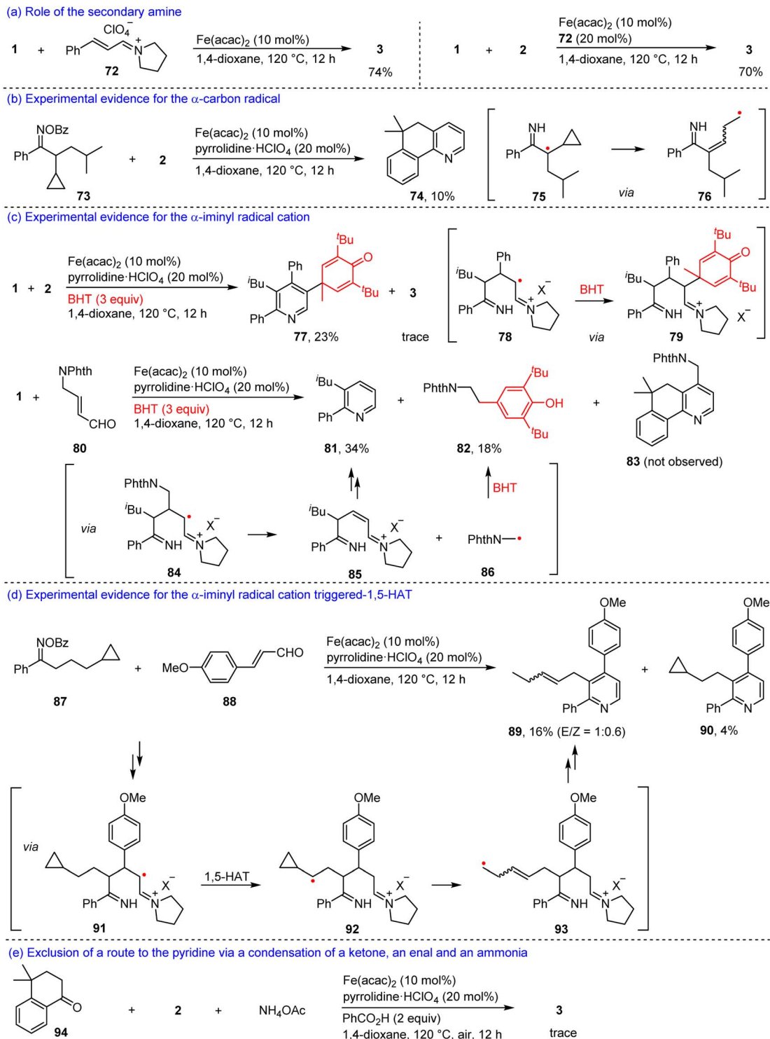
Scheme 6 Mechanistic studies ( X = \text{ClO}_4 , OBz, or acac).
