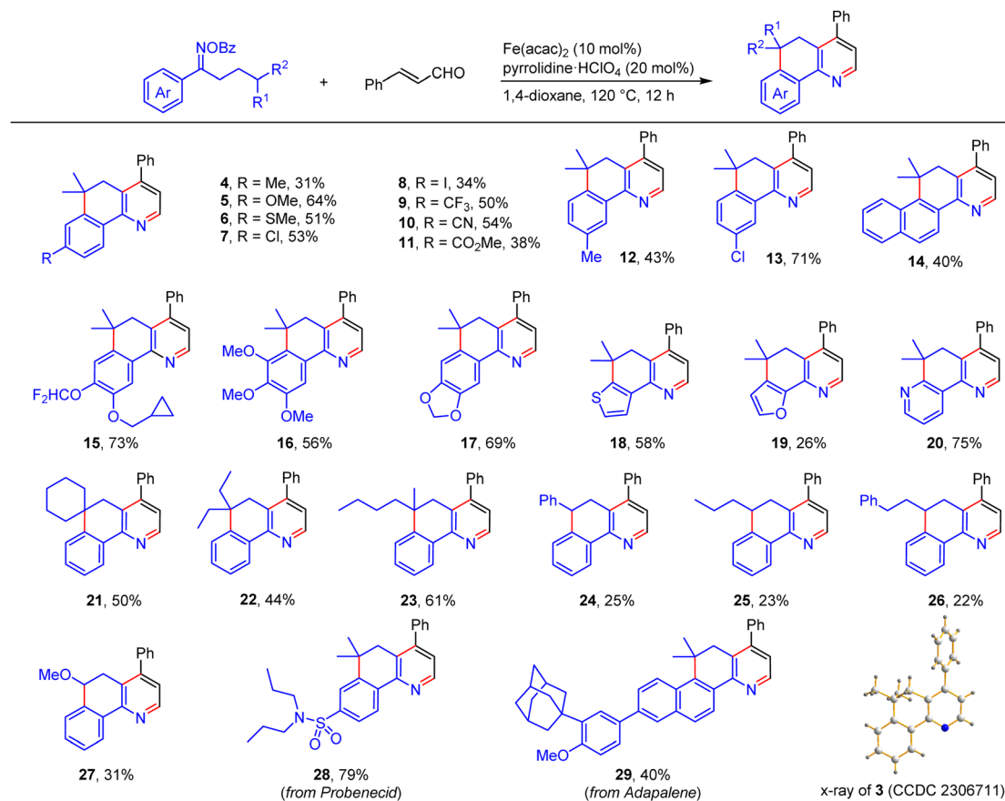
Scheme 3 Substrate scope of the oxime esters. Reaction conditions: oxime ester (0.6 mmol), enal (0.2 mmol), \text{Fe}(\text{acac})_3 (10 mol%), pyrrolidine· \text{HClO}_4 (20 mol%), 1,4-dioxane (2 mL), 120 °C, 12 h, under \text{N}_2 .
