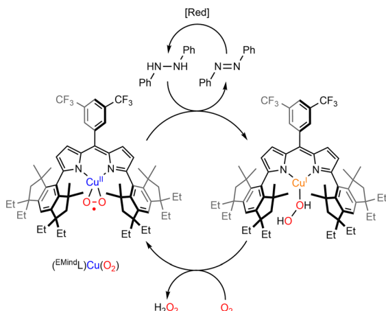
Scheme 7 Reaction of [(\text{EMindL})\text{Cu}^{\text{II}}(\text{O}_2)] with 1,2-diphenylhydrazine to produce azoarene and [(\text{EMindL})\text{Cu}^{\text{II}}(\text{H}_2\text{O}_2)] . Adapted from ref. 83.
