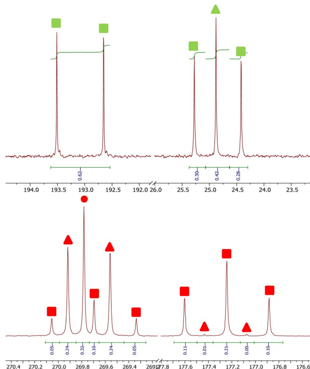
Fig. 16 ^{13}\text{C} containing products from the reaction between 4^{\text{Mes-}^{13}\text{C}} and CO. Top, signals for 8 . Bottom, signals for 2^{\text{Mes}} . Circles signify ^{12}\text{C} products, triangles signify mixed ^{12}\text{C}/^{13}\text{C} and square signifies ^{13}\text{C} products. Markers in green are for ketene ( 8 ) and markers in red are squaraine ( 2^{\text{Mes}} ).
