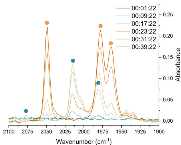
Fig. 1 IR spectra for the first 40 minutes of the reaction between 1^{\text{Mes}} and CO in toluene. CO added to the reaction after six minutes. The colour gradient goes from dark turquoise (earliest) to dark orange (latest). Orange circles highlight the signals for 4^{\text{Mes}} , turquoise circles highlight the signals attributed to 6 .
