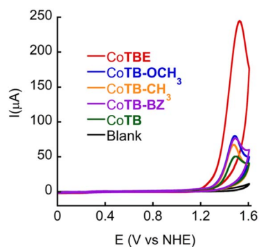
Fig. 8 CV scans of 0.1 M phosphate buffer solution at pH 7 in the absence of a catalyst and in the presence of 0.5 mM CoTBE, CoTB-OCH 3 , CoTB-CH 3 , CoTB-BZ and CoTB (scan rates = 100 mV s -1 ).
