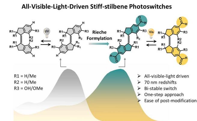
Fig. 1 Molecular structures of the stiff-stilbenes S1 – S6 controlled using UV light and visible light, respectively, and cartoon representation of the absorption band of stiff-stilbenes substituted with aldehydes ( S2 , S4 , and S6 ) and those without formyl group ( S1 , S3 , and S5 ).
