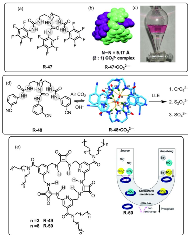
Fig. 16 (a) Chemical structure of the receptor R-47 . (b) Representation of the assembly of R-47·CO 3 2- . (c) Visualization of \text{SO}_4^{2-} extraction using phenolphthalein through the R-47·CO 3 2- complex. (Reproduced from ref. 81. Copyright 2012, The Royal Society of Chemistry.) (d) Schematic representation of LLE by R-48 (Reproduced from ref. 82. Copyright 2014, Wiley.) (e) Chemical structures of the receptors R-49 and R-50 . Illustration of the general setup for the U-tube experiments used to test the ability of R-50 to act as a carrier for \text{SO}_4^{2-} . (Reproduced from ref. 83. Copyright 2020, The Royal Society of Chemistry.)
