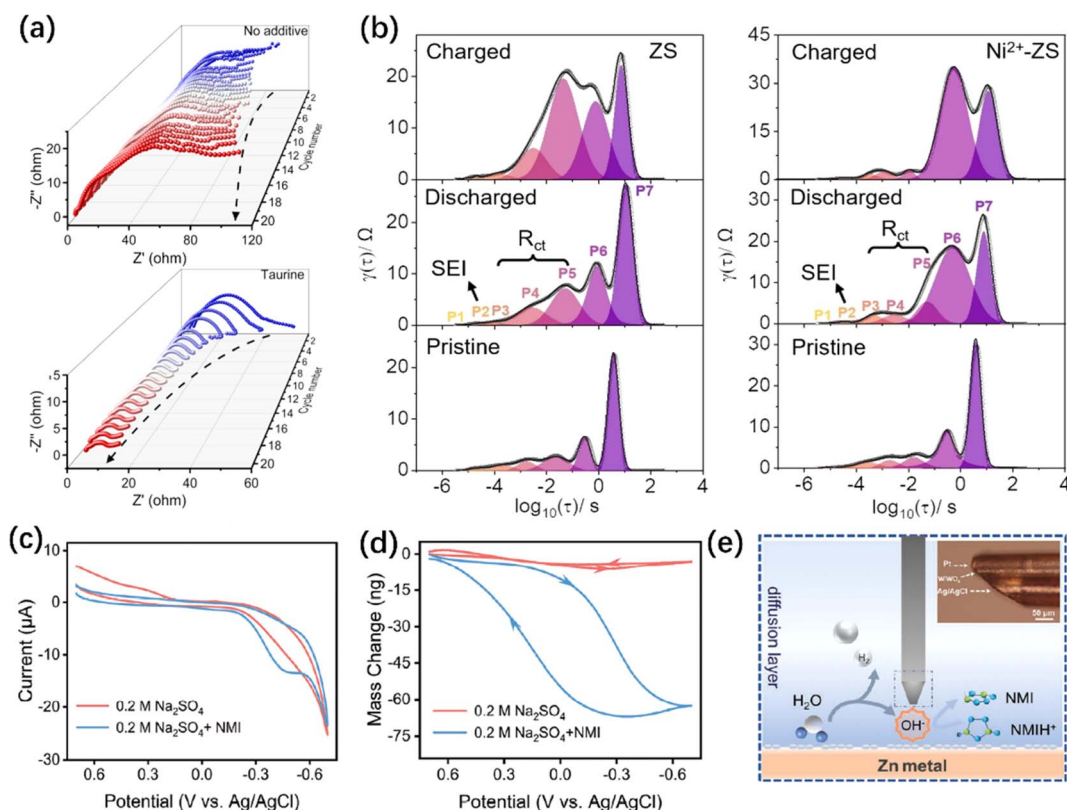
Fig. 9 In situ physicochemical characterizations of ZMA. (a) In situ EIS of symmetrical batteries without/with taurine additive electrolyte. 14 Copyright 2023, Wiley. (b) The distribution of relaxation times (DRT) plot of the in situ EIS data in ZS and \text{Ni}^{2+} –ZS electrolyte. 49 Copyright 2023, Wiley. (c and d) Cyclic voltammograms (CV) curves (c) and corresponding mass change (d) obtained from EQCM test. 107 Copyright 2023, Wiley. (e) Diagram of UME detecting pH changes (inset is a microscopy image of pH UME). 107 Copyright 2023, Wiley.
