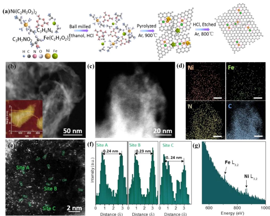
Fig. 24 (a) Schematic illustration of NiFe-DASC synthesis. (b) Dark-field scanning TEM and AFM (inset) images. (c) TEM image and (d) EDS elemental mapping of NiFe-DASC. (e) HAADF-STEM image of NiFe-DASC. (f) Intensity profiles of the three sites in (e). (g) Electronic energy loss spectroscopy (EELS) of NiFe-DASC. Reproduced with permission. 198 Copyright 2021, Nature.
