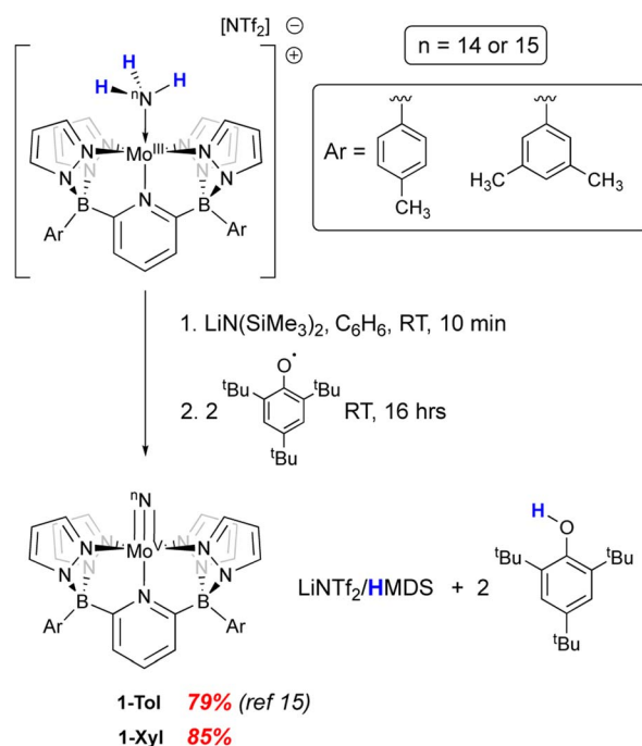
Scheme 2 Synthesis of neutral \text{Mo}(\text{v}) nitrido derivatives 1-Ar ( \text{Ar} = \textit{para} -tolyl, meta -xylyl).
