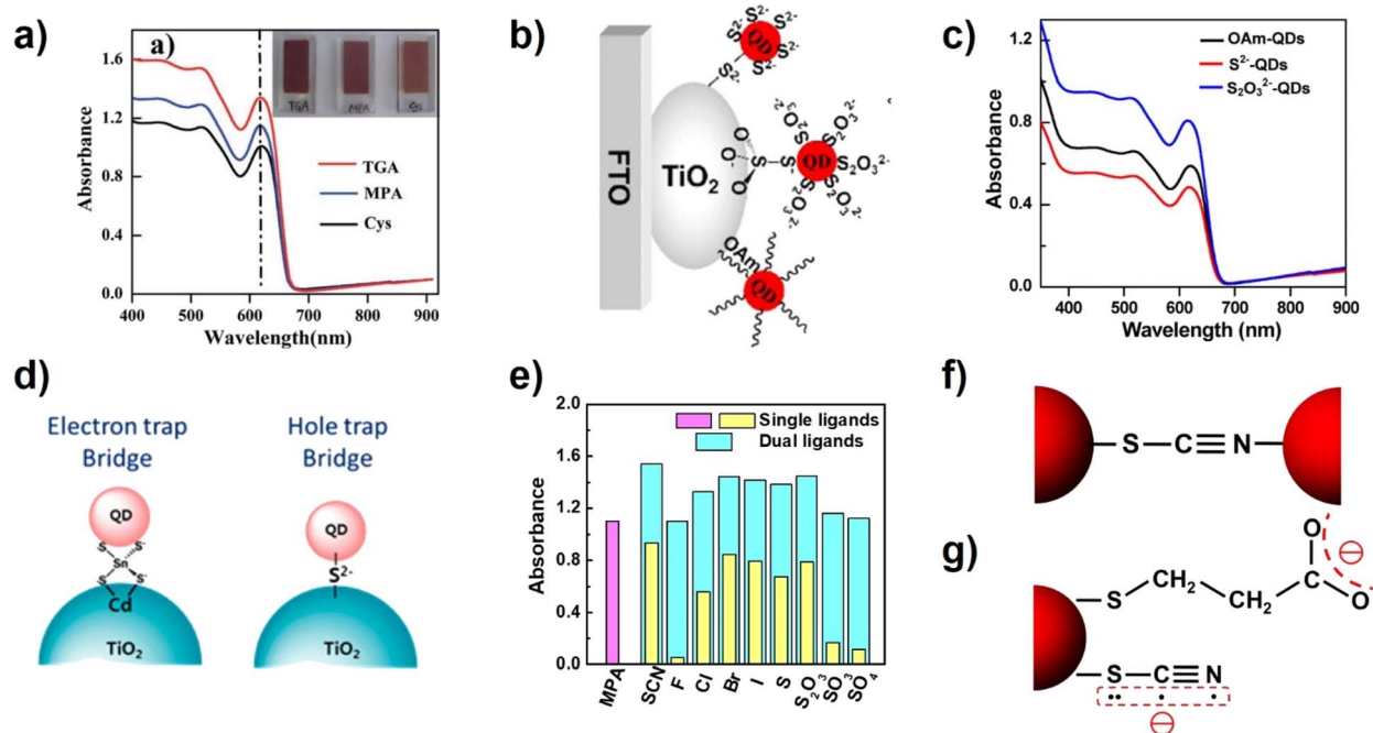
Fig. 6 (a) Absorption spectra of TGA-, MPA-, and Cys-capped CdSe QD sensitized TiO 2 films. (Inset): photographs of films sensitized with different molecules linked to CdSe. 91 This figure has been adapted/reproduced from ref. 91 with permission from The Royal Society of Chemistry, copyright 2014. (b) Schematic diagram and (c) absorption spectra of OAm-, S 2- -, and S 2 O 3 2- -capped CdSe QDs adsorbed on TiO 2 . 94 This figure has been adapted/reproduced from ref. 94 with permission from American Chemical Society, copyright 2017. (d) Illustration of the SnS 4 4- and S 2- ligand-capped QD anchored TiO 2 photoanode. 74 This figure has been adapted/reproduced from ref. 74 with permission from American Chemical Society, copyright 2014. (e) Summary of absorbance values at the wavelength of 600 nm from the absorption spectra of QD-sensitized TiO 2 films, and (f) the possible bidentate bonding motif of the SCN - ligand acting as a crosslinker for two adjacent QDs. (g) Schematics of the molecular structure and charge distribution of MPA and SCN - ligands on the QD surface. 35 The figure has been adapted/reproduced from ref. 35 with permission from American Chemical Society, copyright 2022.
