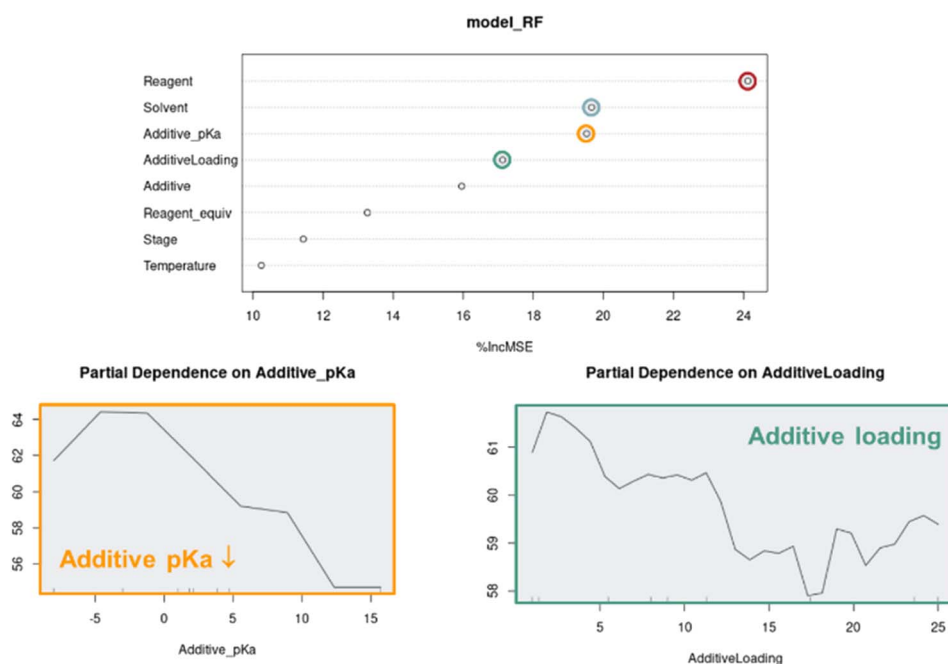
Fig. 12 Random forest (RF) model of the combined autonomous optimization data ranking of parameter influences and partial dependence plots of predicted product 2 UPLC area % on additive \text{p}K_{\text{a}} and loading.
