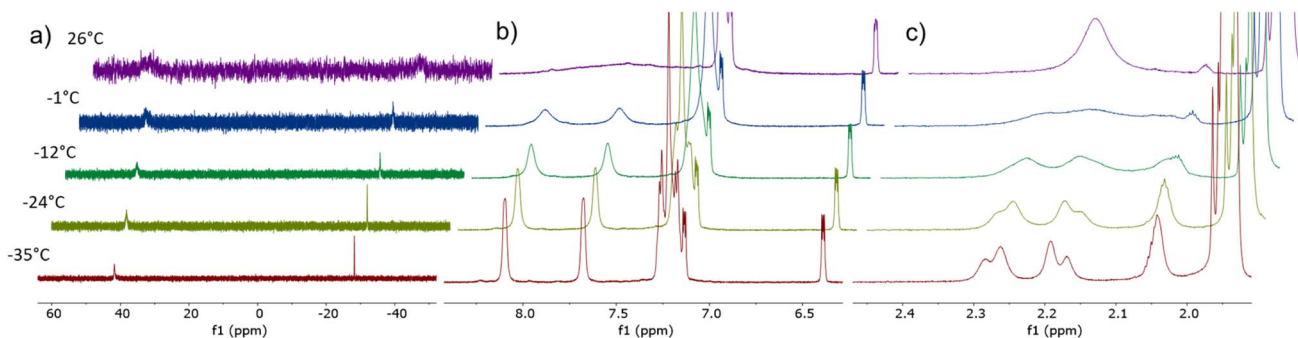
Fig. 4 Variable temperature overlay of: (a) 600 MHz 31 P- 1 H NMR spectra of [Co(triphos)(bdt)][K(18-crown-6)] in acetonitrile- d 3 ; 600 MHz 1 H NMR spectra of [Co(triphos)(bdt)] - in (b) aromatic and (c) aliphatic region in acetonitrile- d 3 . Temperature varied between 26 and -35 °C.
