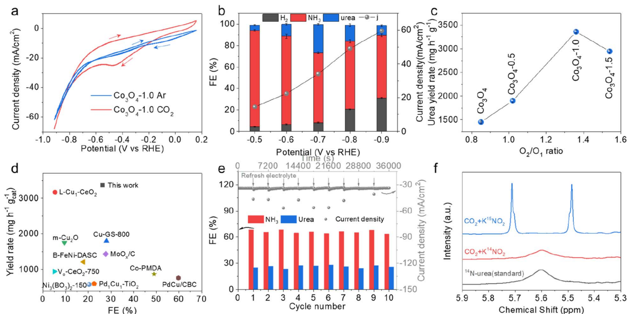
Fig. 2 (a) CV curves of \text{Co}_3\text{O}_4-1.0 at the scan rate of 50 \text{ mV s}^{-1} in Ar or \text{CO}_2 saturated electrolyte. (b) The FE of major products and total current densities over the \text{Co}_3\text{O}_4-1.0 electrocatalyst in \text{CO}_2 saturated 0.2 \text{ M KHCO}_3 + 0.02 \text{ M KNO}_2 electrolyte. (c) The urea yield rate vs. the ratio of \text{O}_2/\text{O}_1 at the potential of -0.7 \text{ V} (vs. RHE). (d) Comparison of the FE (%) of urea and yield rate ( \text{mg h}^{-1} \text{ g}_{\text{cat}}^{-1} ) of \text{Co}_3\text{O}_4-1.0 with those of state-of-the-art catalysts for application in urea synthesis. (e) Stability tests of \text{Co}_3\text{O}_4-1.0 at the potential of -0.7 \text{ V} (vs. RHE). (f) ^1\text{H} NMR spectra obtained by using \text{K}^{14}\text{NO}_2 and \text{K}^{15}\text{NO}_2 as the reactants with \text{CO}_2 and a standard ^{14}\text{N} -urea sample.
