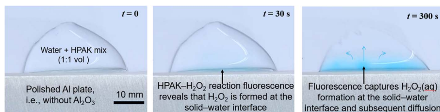
Fig. 3 Time-dependent formation of H 2 O 2 (aq) in a macroscopic droplet of a 1 : 1 mixture of water and HPAK reaction mixture on an Al plate (see ESI Movie S1†). Within seconds, H 2 O 2 (aq) formation at the Al–water interface is evident, proving that the size of the droplet and air–water interface do not matter. The solid–water interface drives this chemical transformation. The Al surface is superhydrophilic, and water spreads on it as a film. Therefore, the Al plate was placed vertically on a polystyrene sheet and formed a 1 ml droplet resting on the Al edge. The 1 : 1 mixture of water and HPAK reaction on polystyrene did not yield the faintest blue fluorescence visible to the naked eye.
