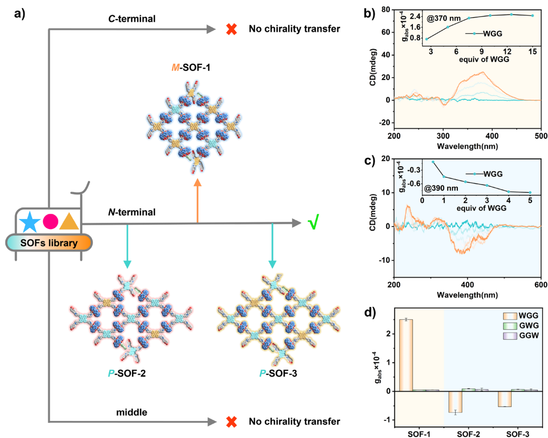
Fig. 5 (a) Schematic representation of the sequence selectivity of SOFs for the guests. CD spectra of (b) SOF-1 and (c) SOF-2 with WGG in \text{H}_2\text{O} . (d) g_{\text{abs}} intensities of SOF-1, SOF-2, and SOF-3 with WGG, GWG, and GGW. SOF-1 is monitored at 370 nm; SOF-2 and SOF-3 at 390 nm.
