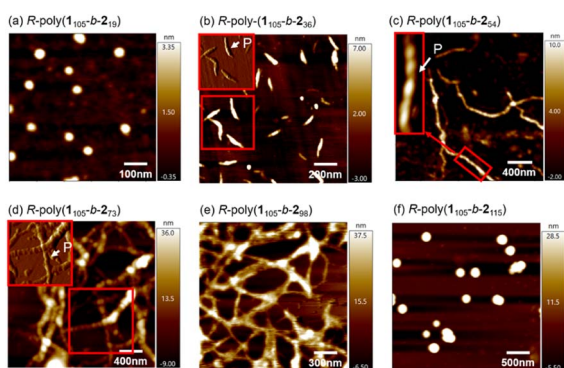
Fig. 5 AFM images of R -poly( 1 105 - b - 2 19 ) (a), R -poly( 1 105 - b - 2 36 ) (b), R -poly( 1 105 - b - 2 54 ) (c), R -poly( 1 105 - b - 2 73 ) (d), and R -poly( 1 105 - b - 2 98 ) (e), and R -poly( 1 105 - b - 2 115 ) (f).
