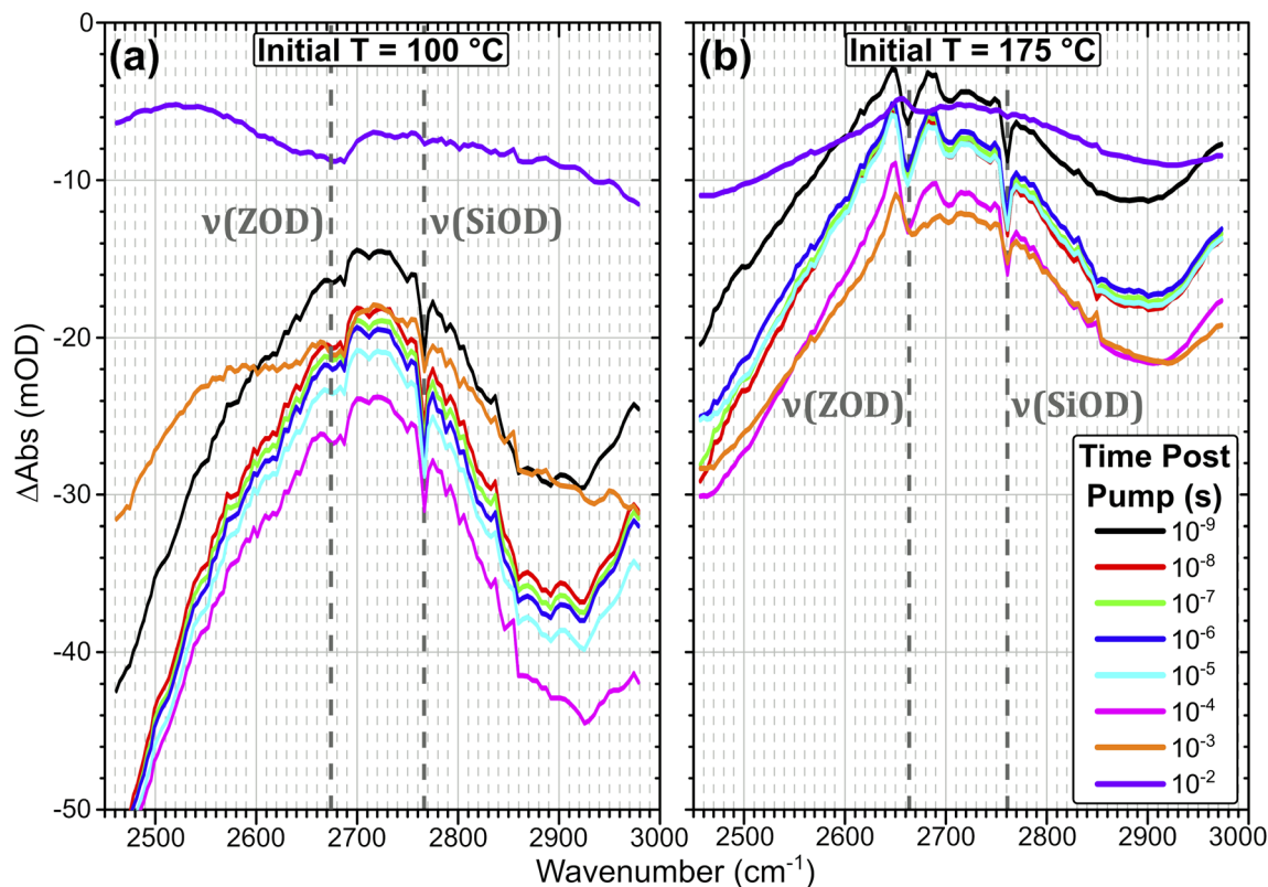
Fig. 4 Time-resolved IR spectral evolution of ZSM-5 in flowing HOD/H _2 O vapour at an initial temperature of 100^\circ\text{C} (a) and 175^\circ\text{C} (b). Spectra are shown at logarithmic time intervals from 10^{-9} – 10^{-2} s following pumping with the 70\text{ }\mu\text{J} laser pulse. The \nu(\text{SiOD}) silanol modes and free \nu(\text{OD}) Brønsted acid modes are highlighted.
