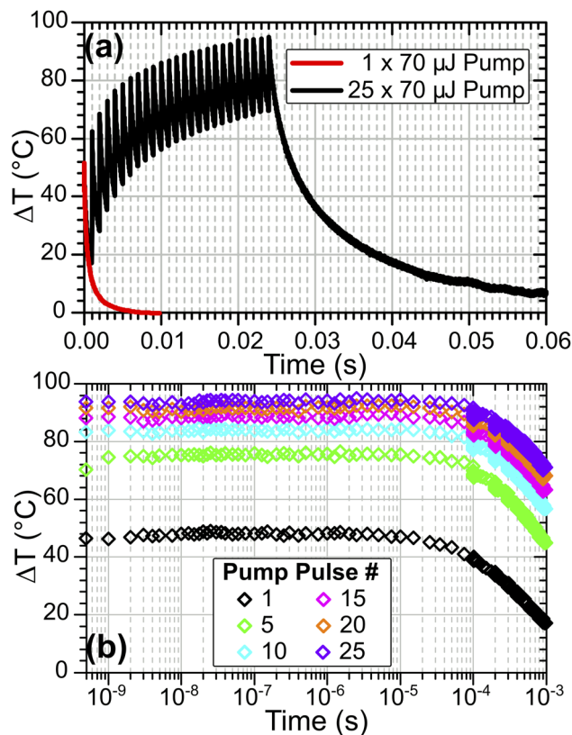
Fig. 11 (a) Sample temperature evolution for HOD/H 2 O in ZSM-5 at T_{\text{init}} = 125 °C following pumping by 1× (red) and 25× (black) 70 \mu J pump pulses. (b) Comparison of temperature evolution in first 1 ms following indicated pulse number in 25-pulse burst showing nanosecond time resolution throughout full range.
