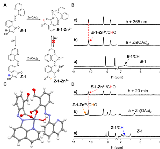
Fig. 4 (A) Illustration of the modulation of E -1 with coordination and light. (B) ^1\text{H} NMR spectra of E -1 in \text{DMSO}-d_6 (10 mM, a), its mixture with \text{Zn}(\text{OAc})_2 \cdot 2\text{H}_2\text{O} (1.5 equiv., b), and after irradiation for 1.5 h at 365 nm (c). (C) X-ray structure of E -1- \text{Zn}^{2+} . (D) ^1\text{H} NMR spectra of Z -enriched solution of 1 (created by irradiation of E -1 for 1.5 h at 365 nm) in \text{DMSO}-d_6 (10 mM, a), its mixture with \text{Zn}(\text{OAc})_2 \cdot 2\text{H}_2\text{O} (2.5 equiv., b), and after 20 min (c).
